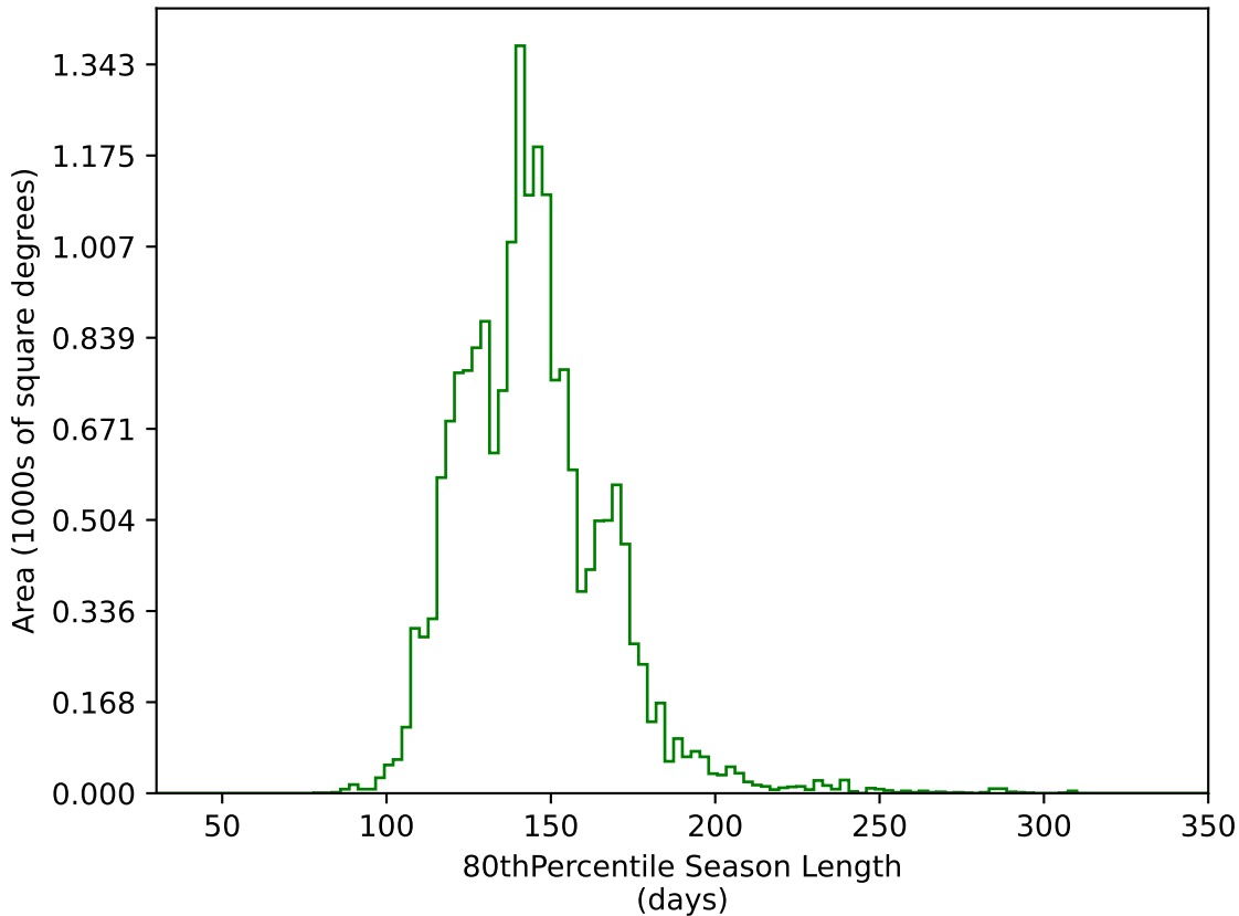
weather_cloudso6v3.4_10yrs WFD g band: 80thPercentile Season Length
