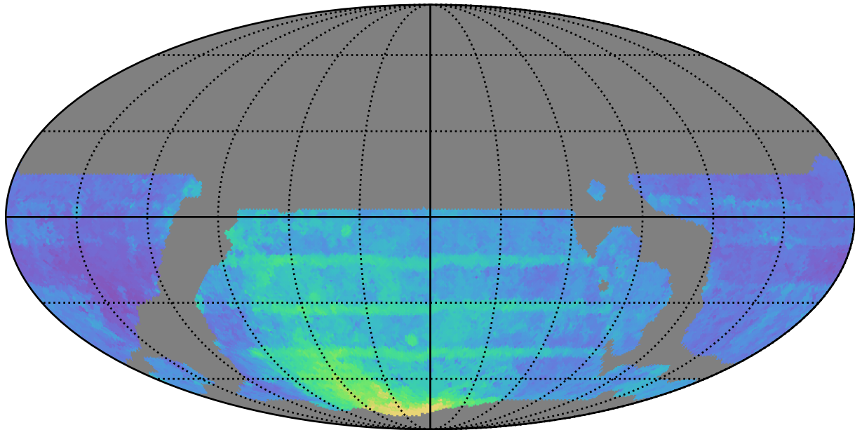
weather_cloudso6v3.4_10yrs WFD all bands: 80thPercentile Season Length
