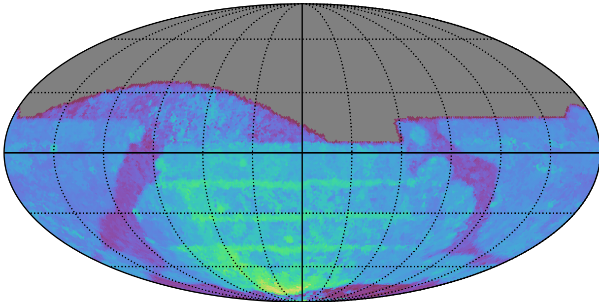
weather_cloudso6v3.4_10yrs All sky z band: 80thPercentile Season Length
