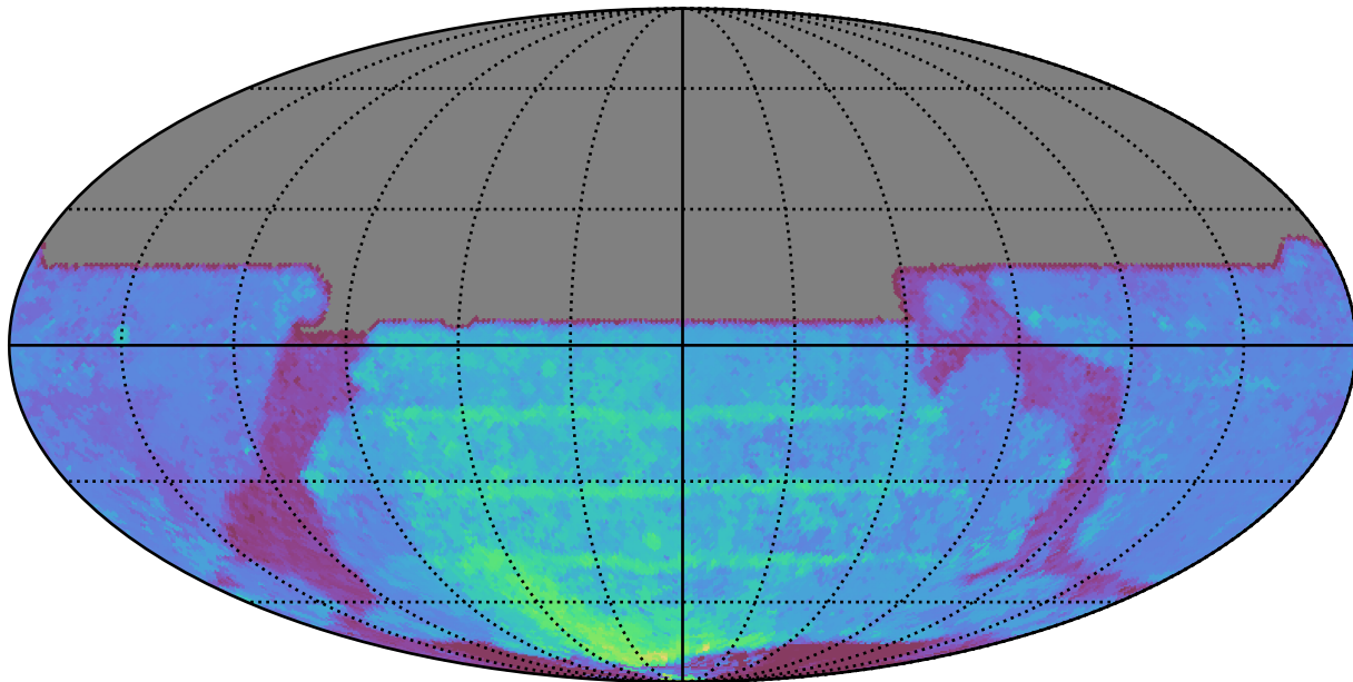
weather_cloudso6v3.4_10yrs All sky y band: 80thPercentile Season Length
