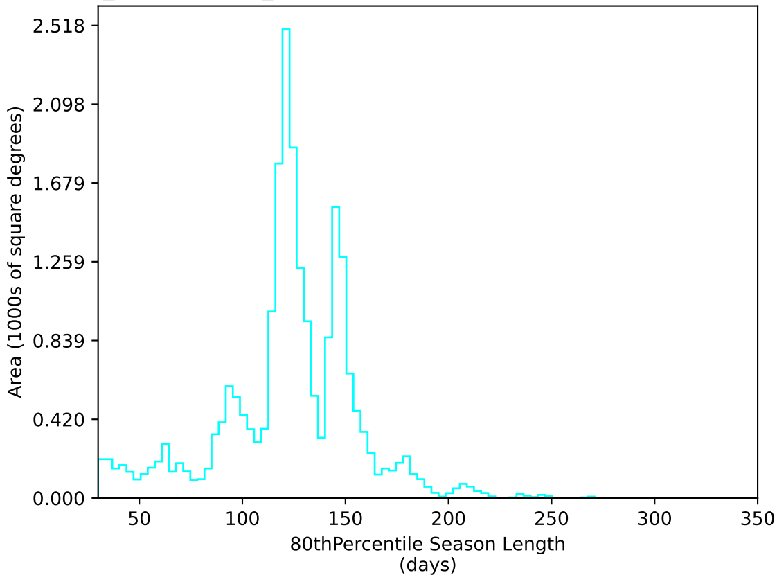
weather_cloudso6v3.4_10yrs All sky u band: 80thPercentile Season Length
