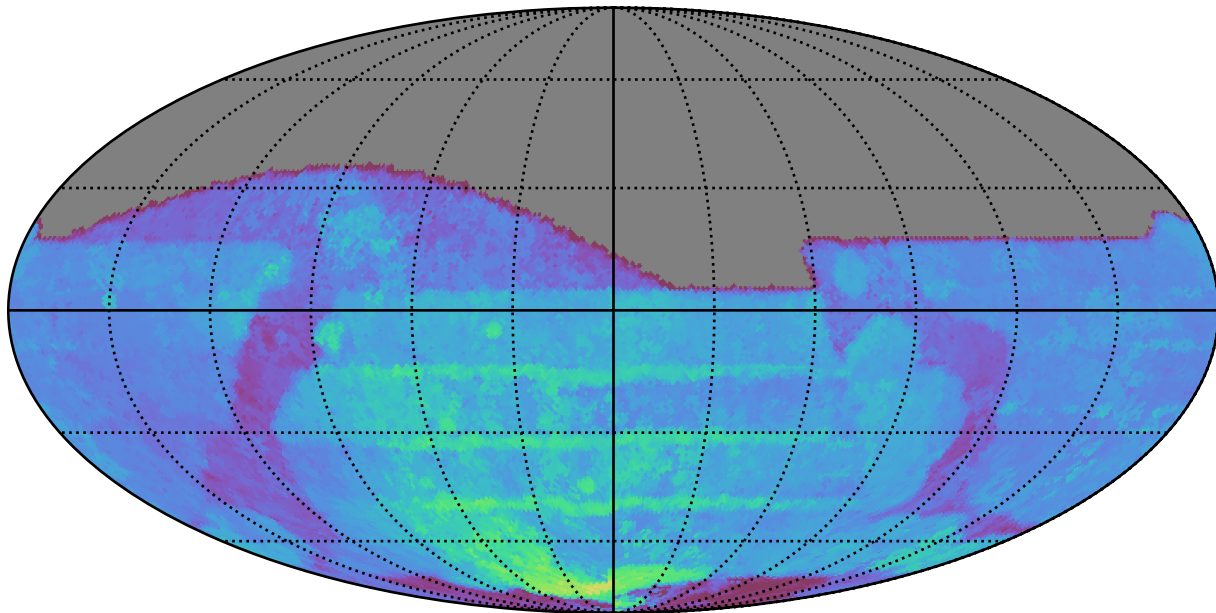
weather_cloudso6v3.4_10yrs All sky r band: 80thPercentile Season Length
