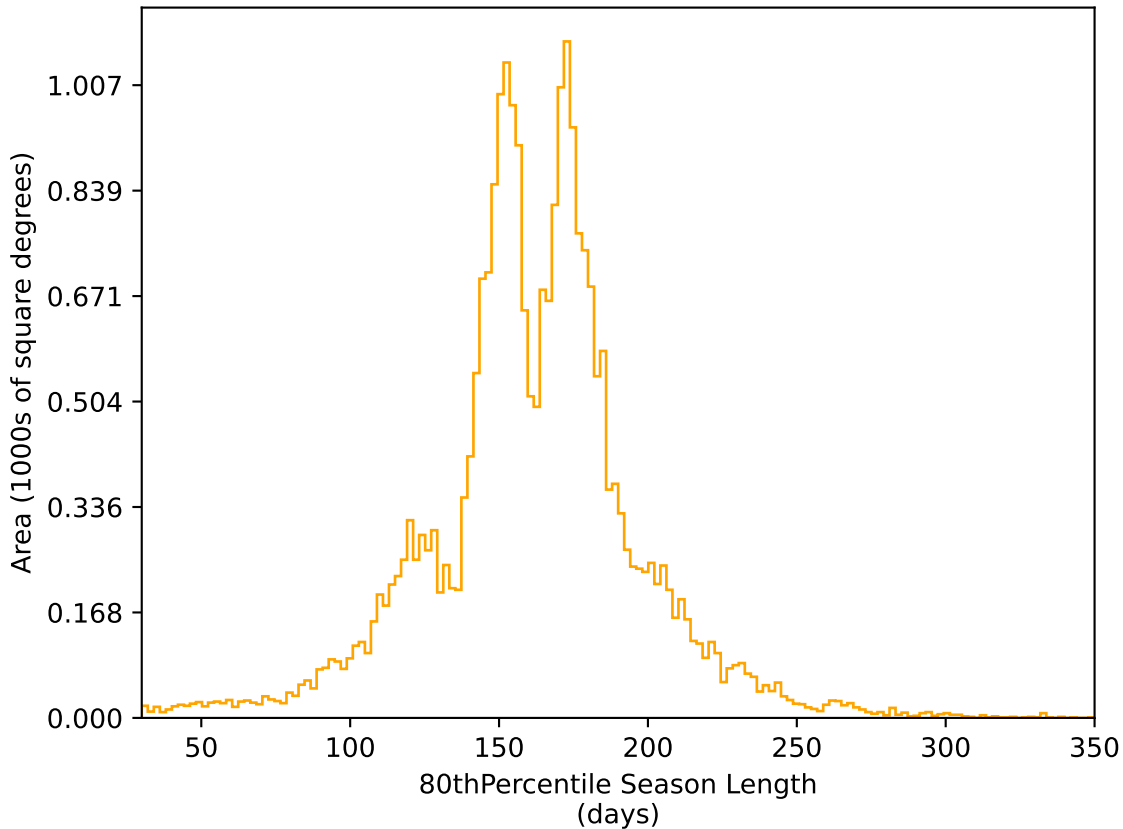
weather_cloudso6v3.4_10yrs All sky r band: 80thPercentile Season Length
