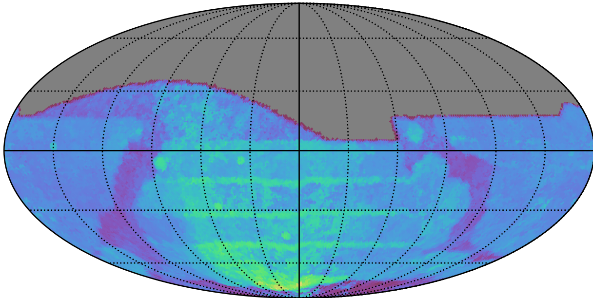
weather_cloudso6v3.4_10yrs All sky i band: 80thPercentile Season Length
