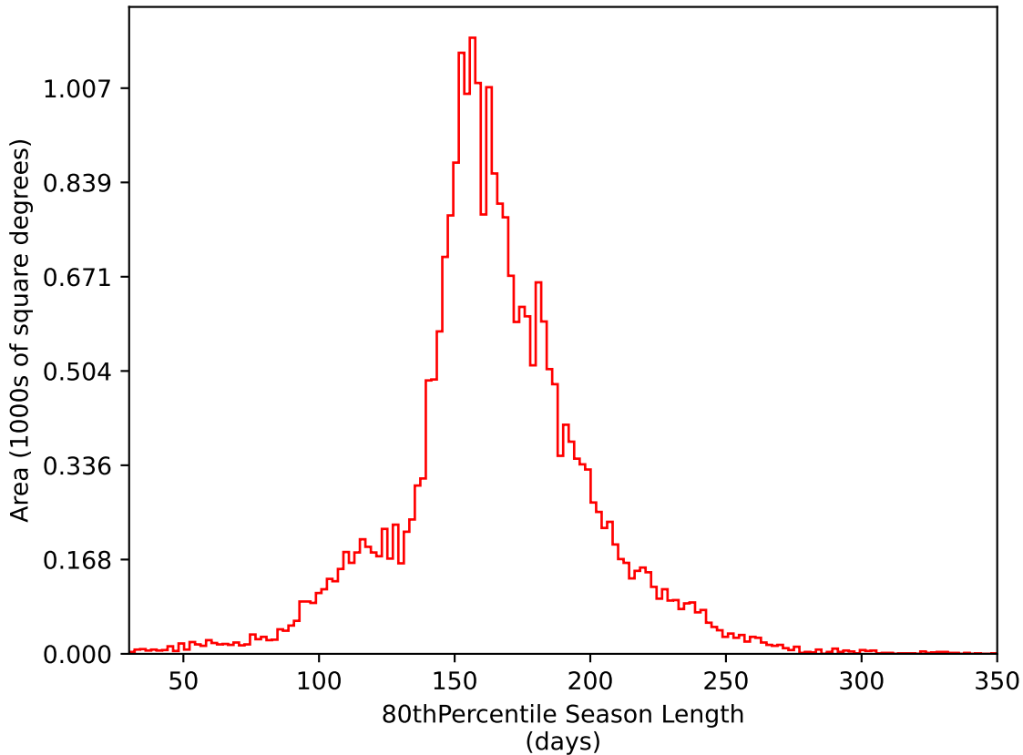
weather_cloudso6v3.4_10yrs All sky i band: 80thPercentile Season Length
