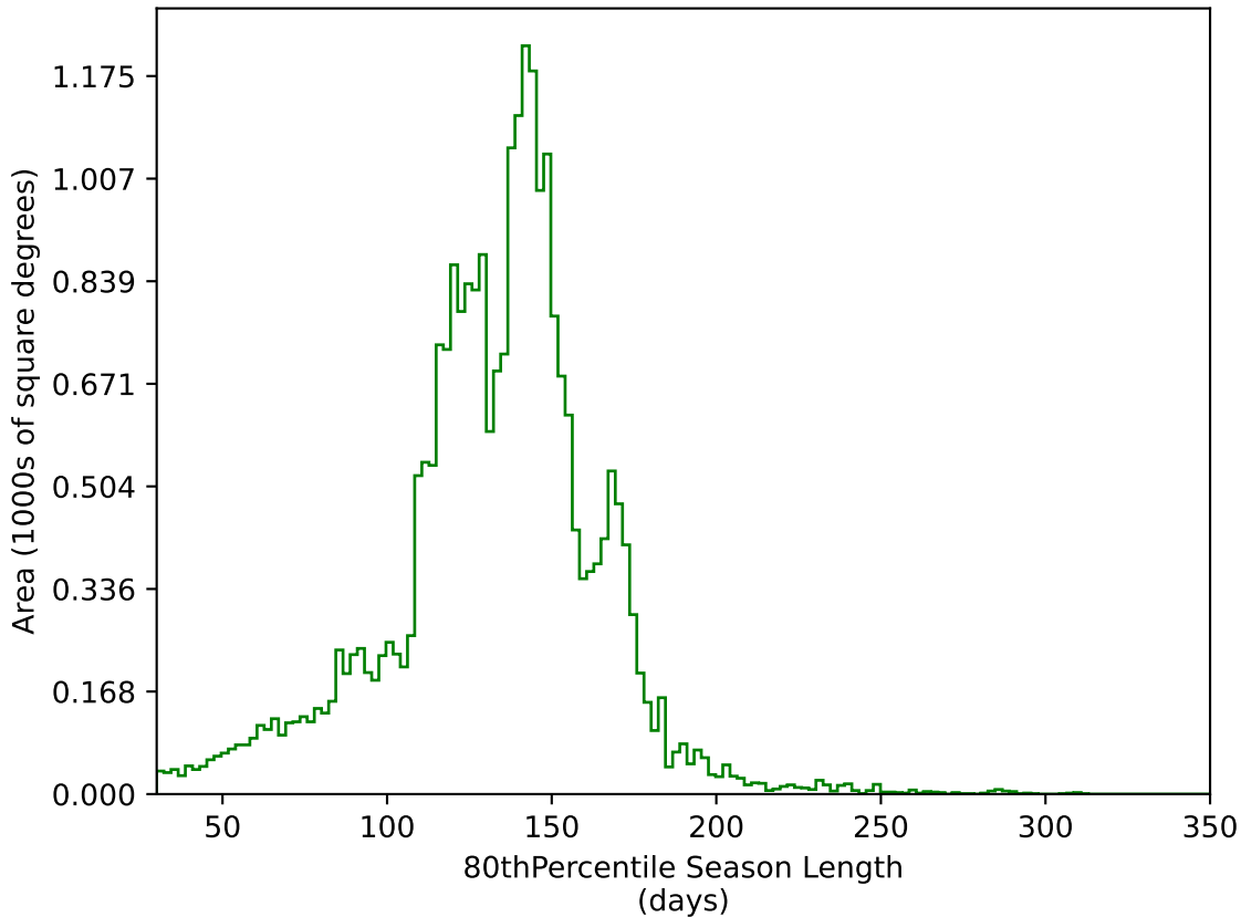
weather_cloudso6v3.4_10yrs All sky g band: 80thPercentile Season Length
