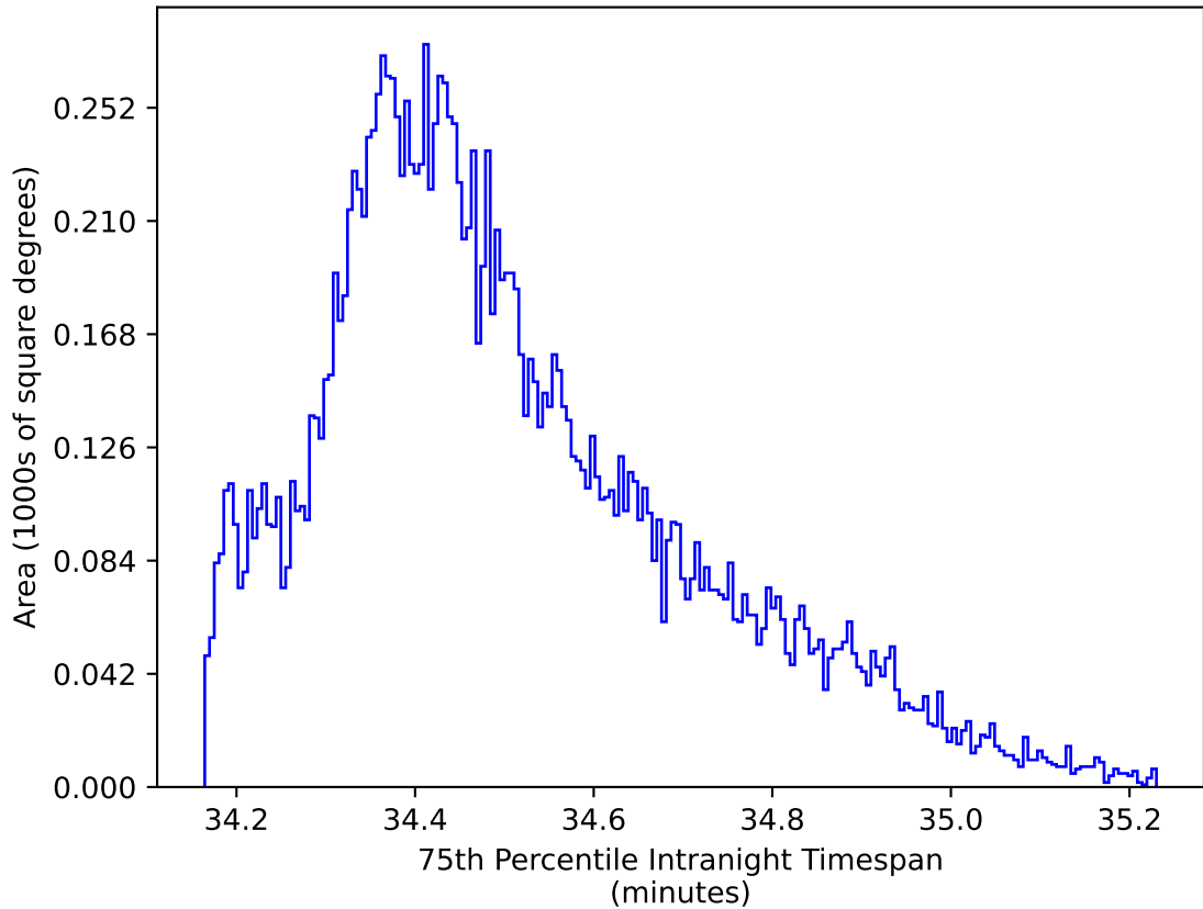
weather_cloudso6v3.4_10yrs WFD zy bands: 75th Percentile Intranight Timespan
