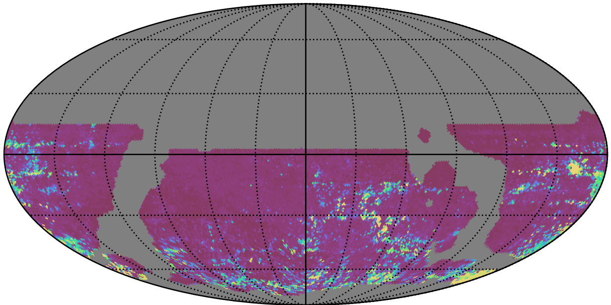
weather_cloudso6v3.4_10yrs WFD z band: 75th Percentile Intranight Timespan
