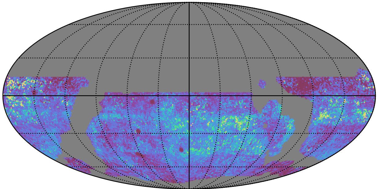
weather_cloudso6v3.4_10yrs WFD y band: 75th Percentile Intranight Timespan
