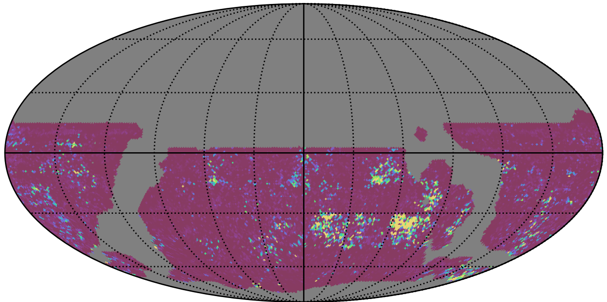
weather_cloudso6v3.4_10yrs WFD u band: 75th Percentile Intranight Timespan
