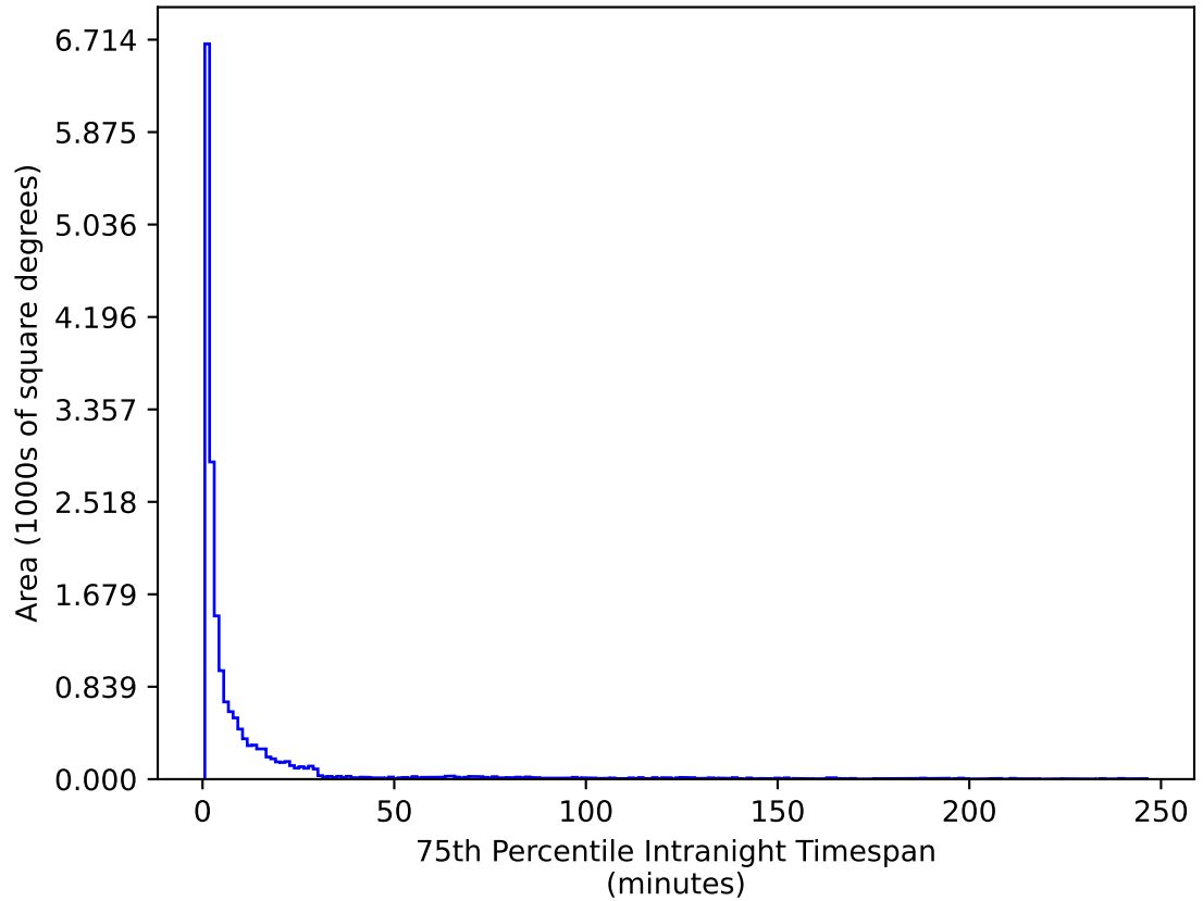
weather_cloudso6v3.4_10yrs WFD u band: 75th Percentile Intranight Timespan
