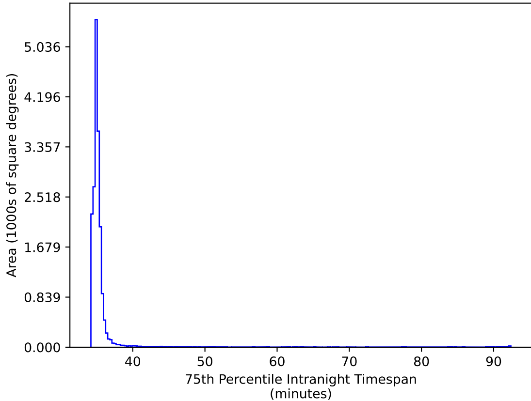
weather_cloudso6v3.4_10yrs WFD ri bands: 75th Percentile Intranight Timespan
