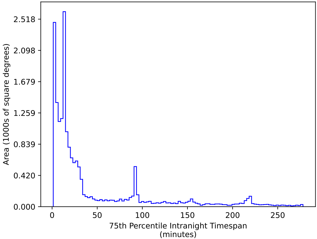
weather_cloudso6v3.4_10yrs WFD r band: 75th Percentile Intranight Timespan
