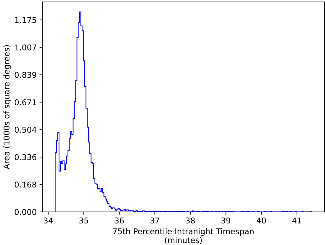
weather_cloudso6v3.4_10yrs WFD iz bands: 75th Percentile Intranight Timespan
