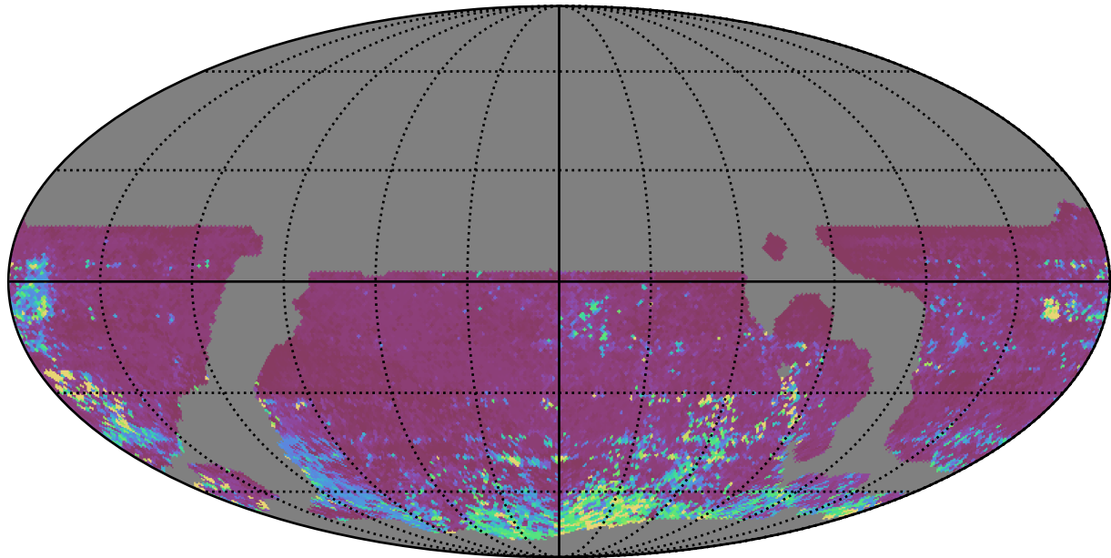
weather_cloudso6v3.4_10yrs WFD i band: 75th Percentile Intranight Timespan
