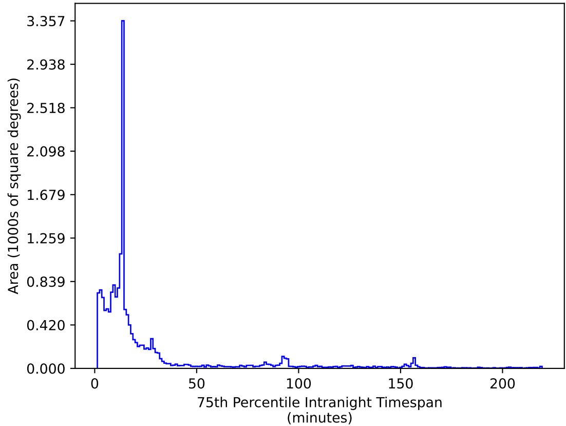
weather_cloudso6v3.4_10yrs WFD i band: 75th Percentile Intranight Timespan
