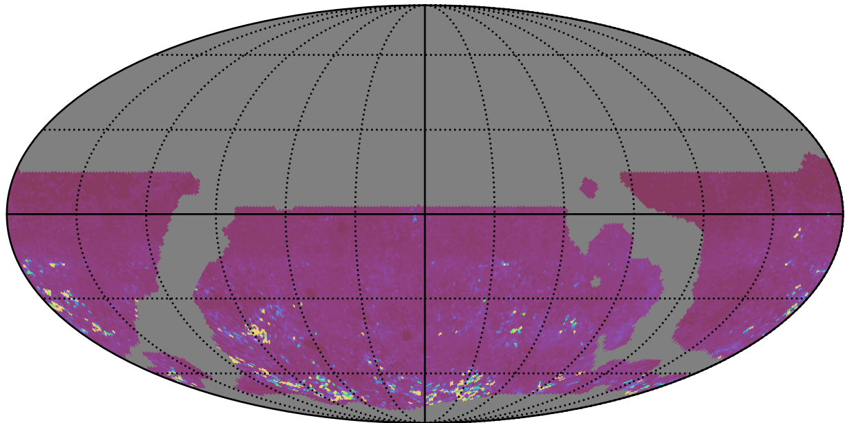
weather_cloudso6v3.4_10yrs WFD gr bands: 75th Percentile Intranight Timespan
