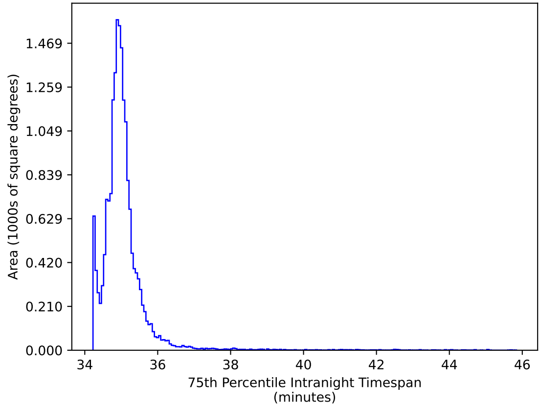
weather_cloudso6v3.4_10yrs WFD gr bands: 75th Percentile Intranight Timespan
