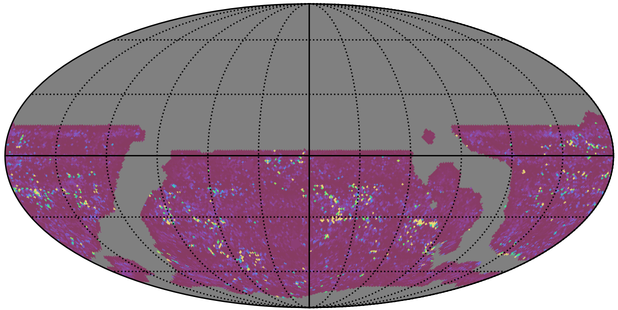
weather_cloudso6v3.4_10yrs WFD g band: 75th Percentile Intranight Timespan
