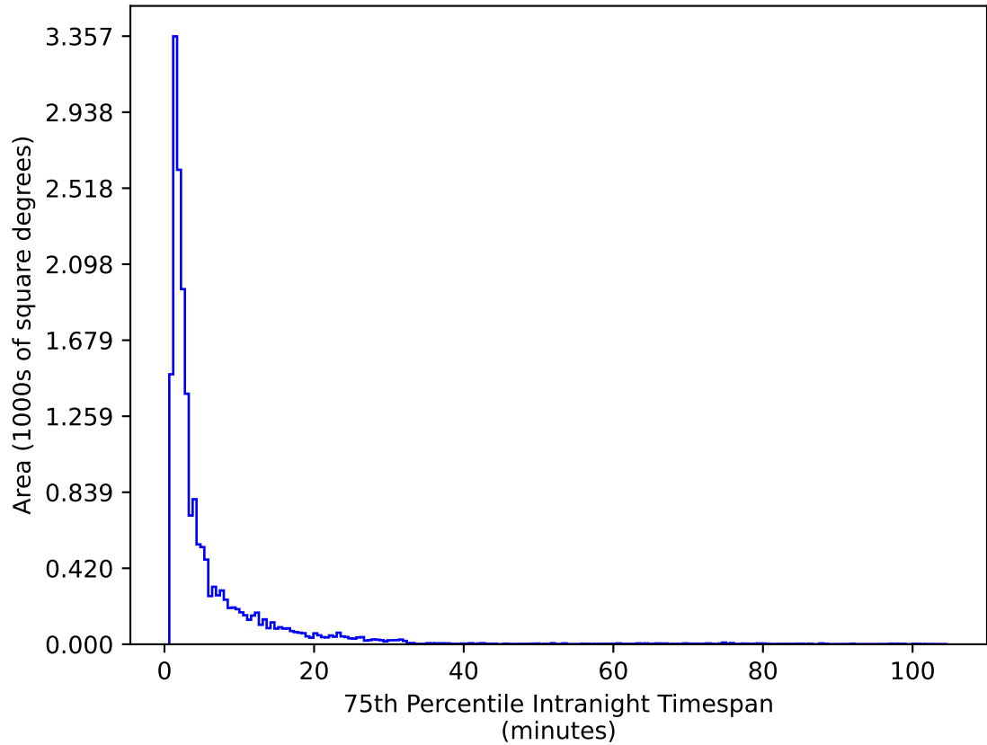
weather_cloudso6v3.4_10yrs WFD g band: 75th Percentile Intranight Timespan
