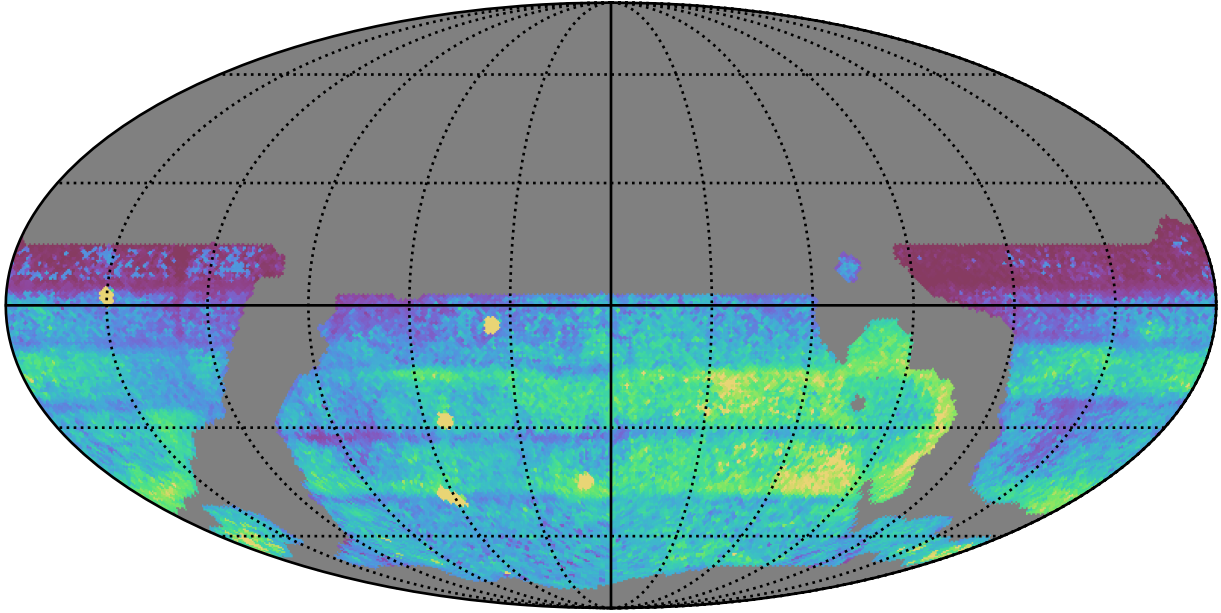
weather_cloudso6v3.4_10yrs WFD all bands: 75th Percentile Intranight Timespan
