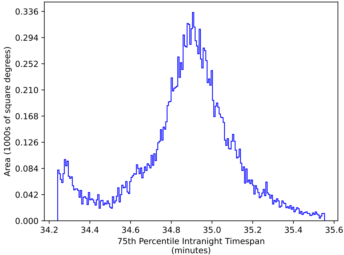
weather_cloudso6v3.4_10yrs WFD all bands: 75th Percentile Intranight Timespan
