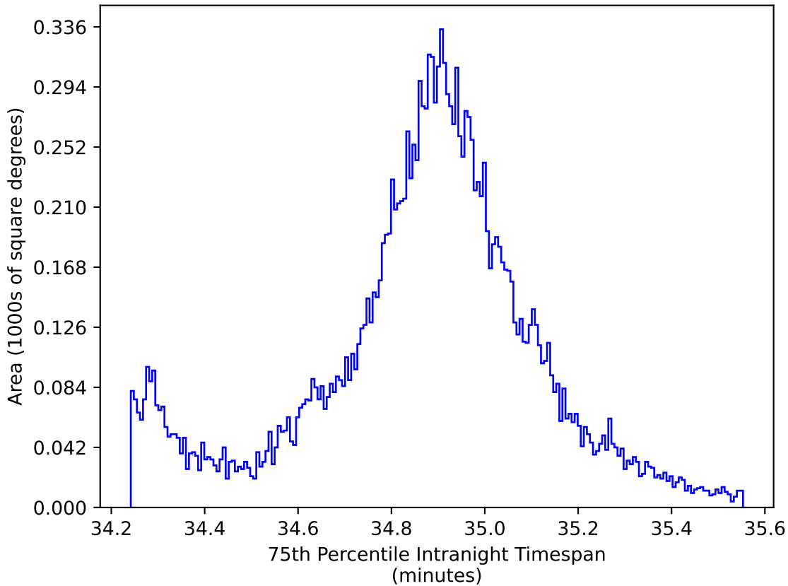
weather_cloudso6v3.4_10yrs WFD: 75th Percentile Intranight Timespan
