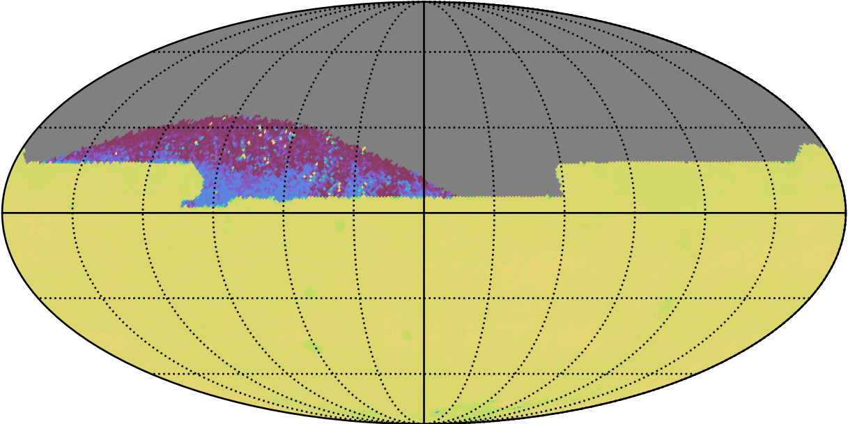
weather_cloudso6v3.4_10yrs All sky zy bands: 75th Percentile Intranight Timespan
