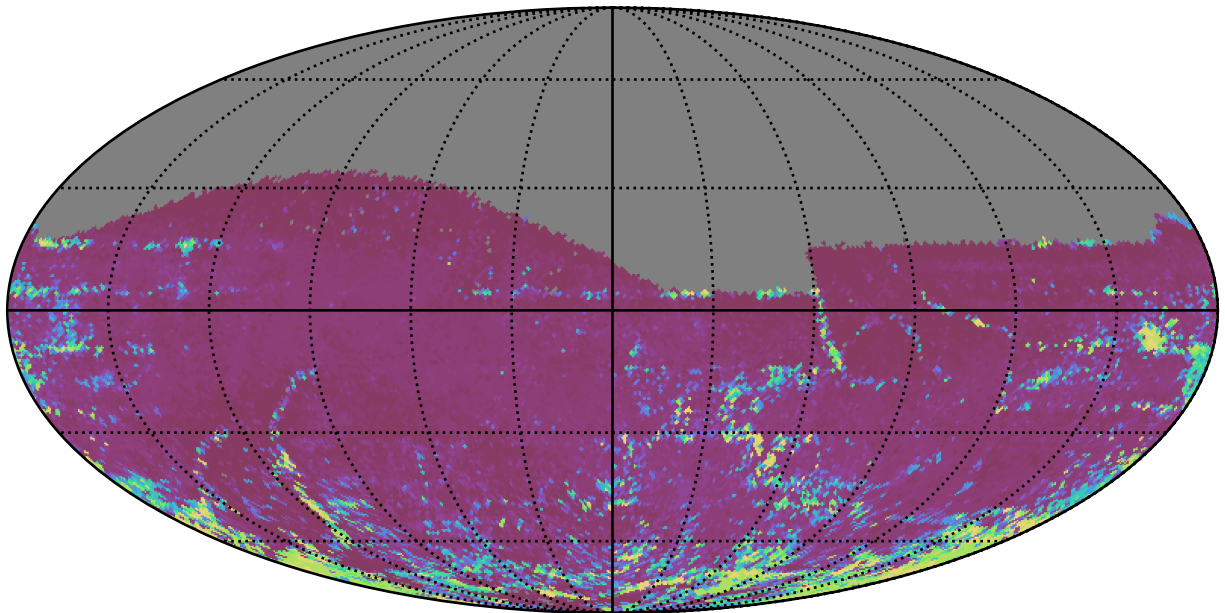
weather_cloudso6v3.4_10yrs All sky z band: 75th Percentile Intranight Timespan
