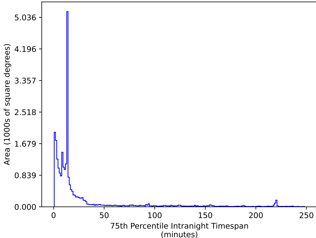
weather_cloudso6v3.4_10yrs All sky z band: 75th Percentile Intranight Timespan
