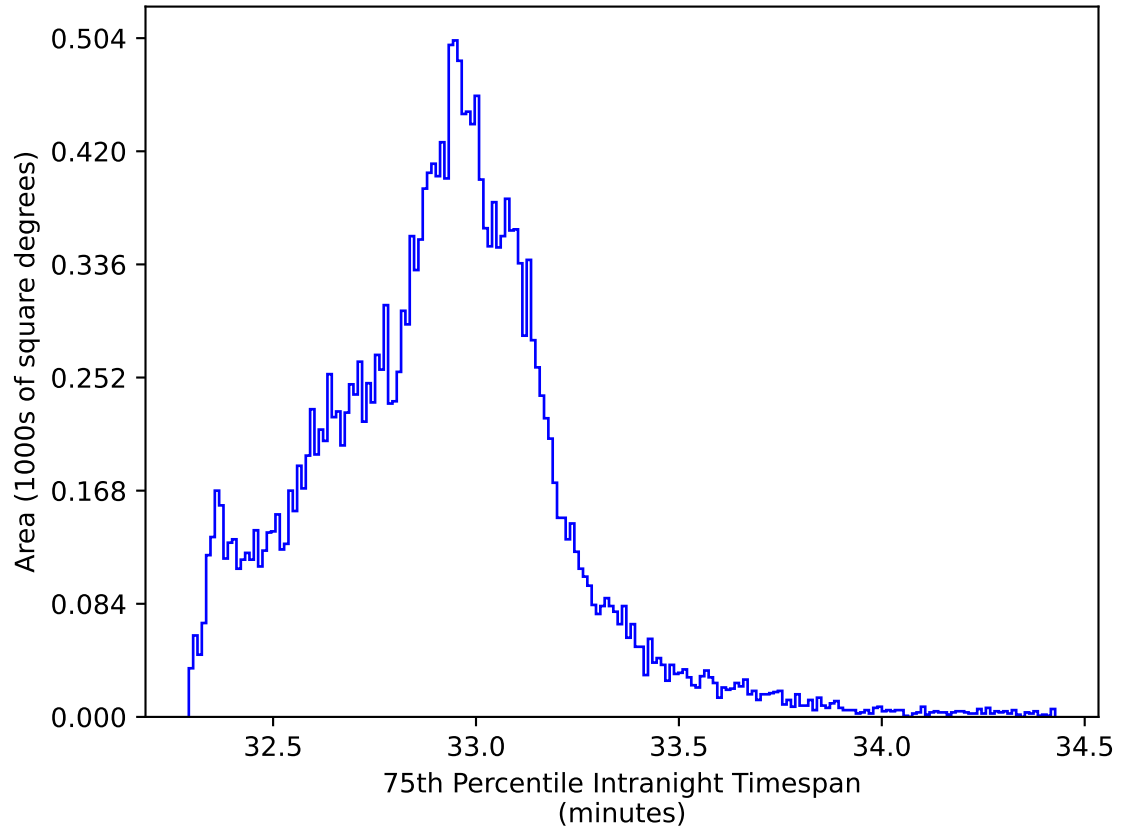
weather_cloudso6v3.4_10yrs All sky y band: 75th Percentile Intranight Timespan
