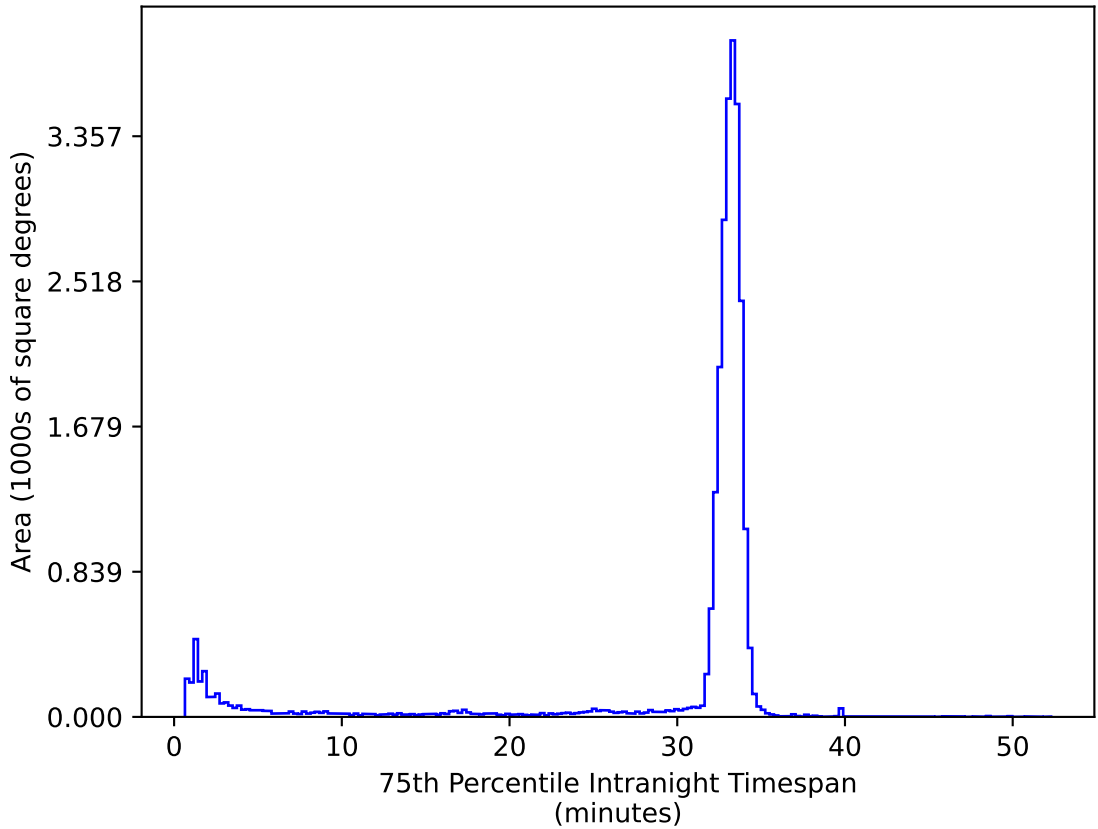
weather_cloudso6v3.4_10yrs All sky ug bands: 75th Percentile Intranight Timespan
