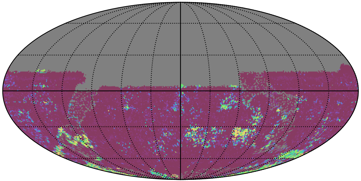
weather_cloudso6v3.4_10yrs All sky u band: 75th Percentile Intranight Timespan
