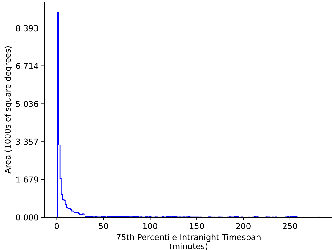
weather_cloudso6v3.4_10yrs All sky u band: 75th Percentile Intranight Timespan
