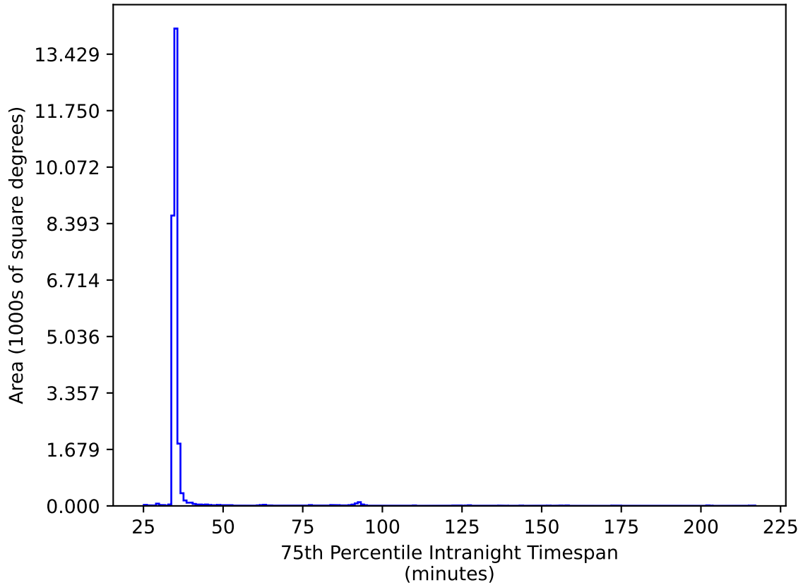
weather_cloudso6v3.4_10yrs All sky ri bands: 75th Percentile Intranight Timespan
