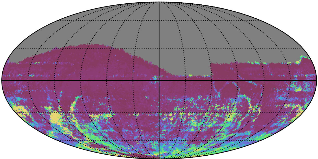
weather_cloudso6v3.4_10yrs All sky r band: 75th Percentile Intranight Timespan
