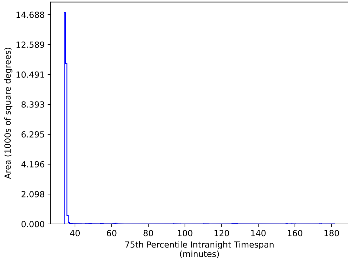
weather_cloudso6v3.4_10yrs All sky iz bands: 75th Percentile Intranight Timespan
