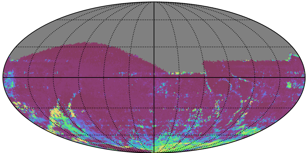
weather_cloudso6v3.4_10yrs All sky i band: 75th Percentile Intranight Timespan
