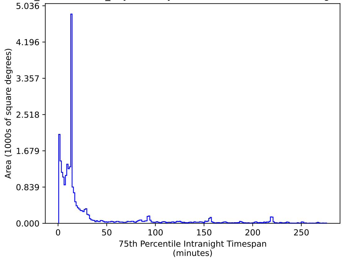
weather_cloudso6v3.4_10yrs All sky i band: 75th Percentile Intranight Timespan
