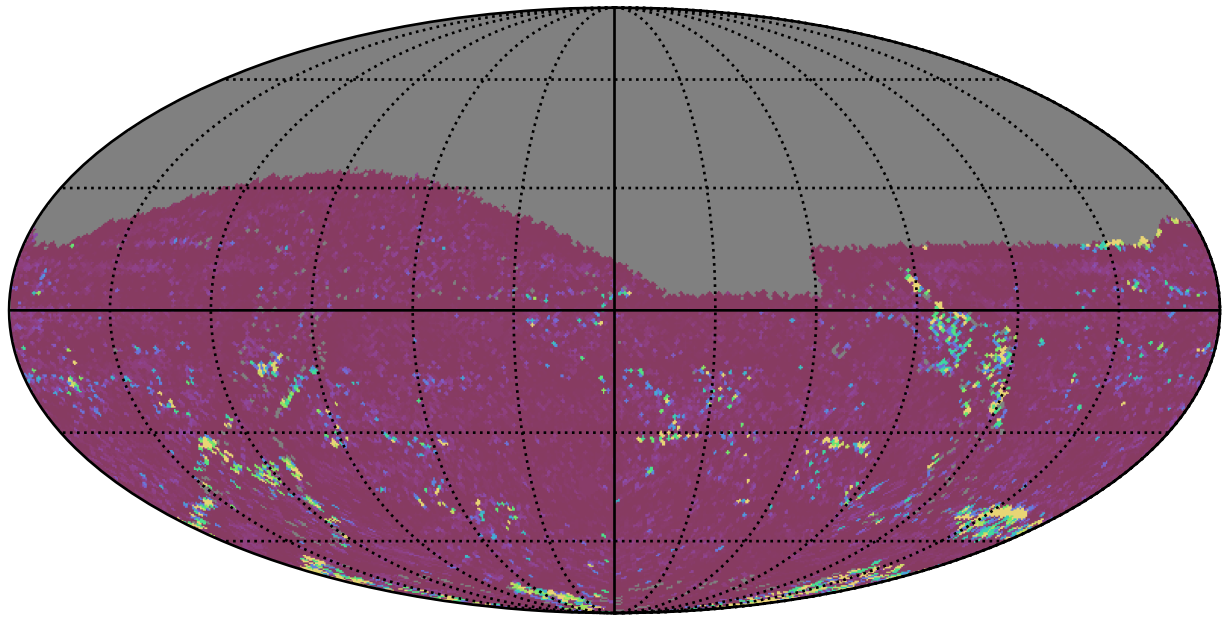
weather_cloudso6v3.4_10yrs All sky g band: 75th Percentile Intranight Timespan
