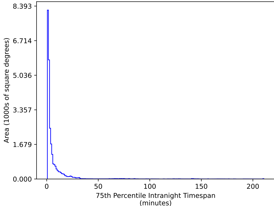
weather_cloudso6v3.4_10yrs All sky g band: 75th Percentile Intranight Timespan
