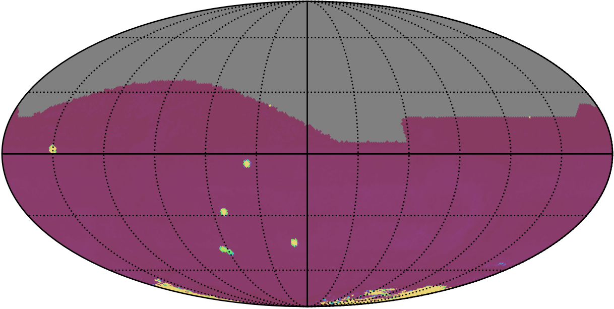
weather_cloudso6v3.4_10yrs All sky all bands: 75th Percentile Intranight Timespan
