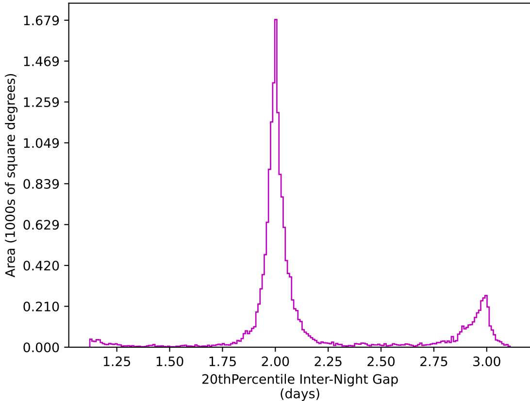
weather_cloudso6v3.4_10yrs WFD z band: 20thPercentile Inter-Night Gap
