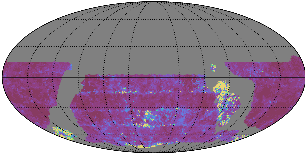
weather_cloudso6v3.4_10yrs WFD u band: 20thPercentile Inter-Night Gap
