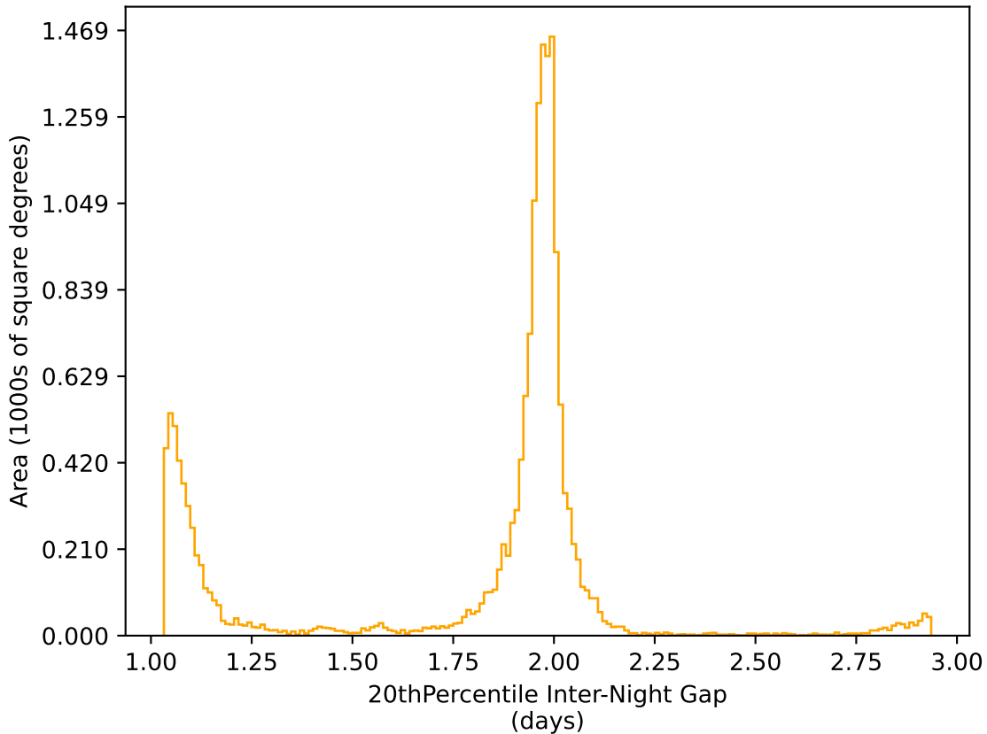
weather_cloudso6v3.4_10yrs WFD r band: 20thPercentile Inter-Night Gap
