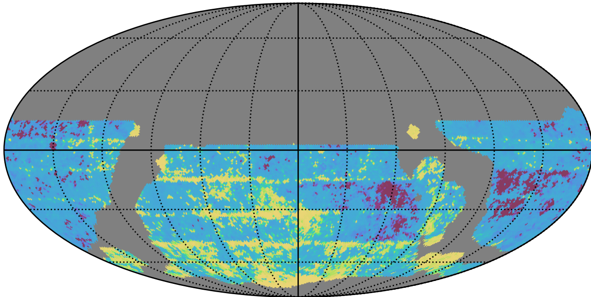
weather_cloudso6v3.4_10yrs WFD i band: 20thPercentile Inter-Night Gap
