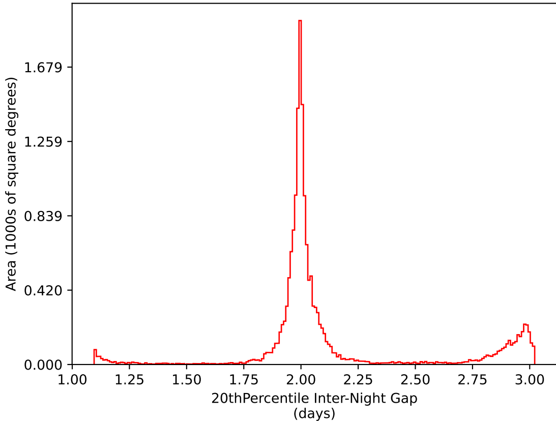
weather_cloudso6v3.4_10yrs WFD i band: 20thPercentile Inter-Night Gap
