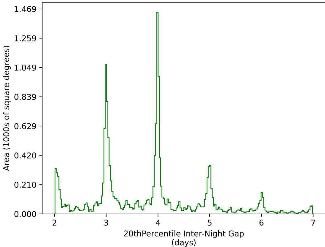
weather_cloudso6v3.4_10yrs WFD g band: 20thPercentile Inter-Night Gap
