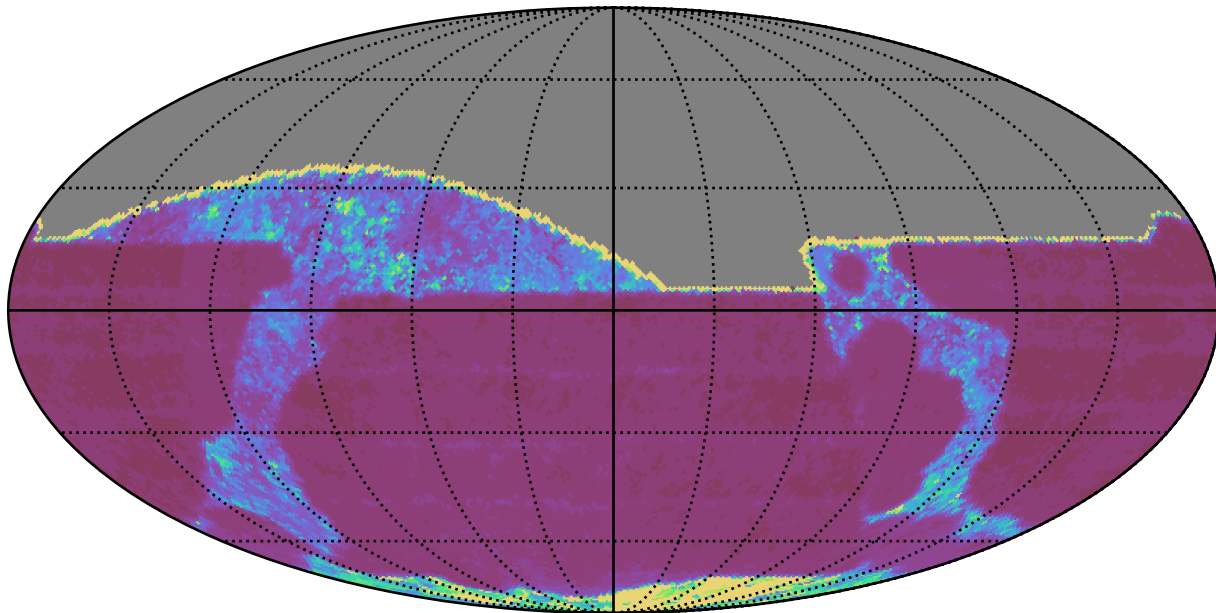
weather_cloudso6v3.4_10yrs All sky r band: 20thPercentile Inter-Night Gap
