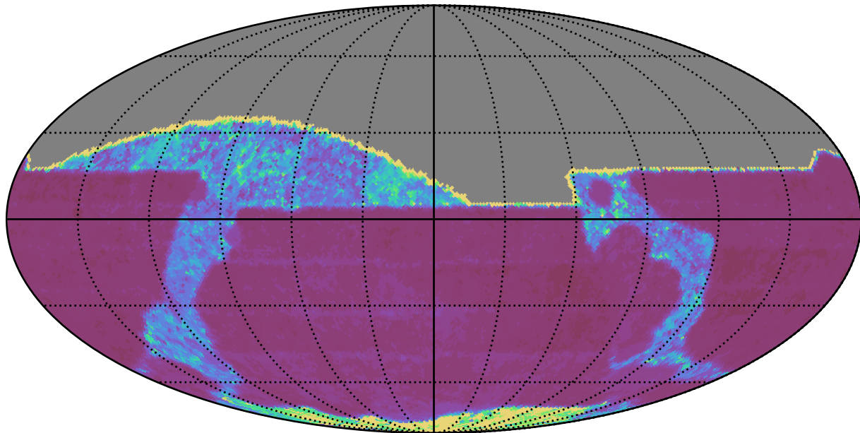
weather_cloudso6v3.4_10yrs All sky i band: 20thPercentile Inter-Night Gap
